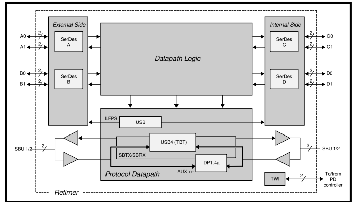
KB8002 Block Diagram
