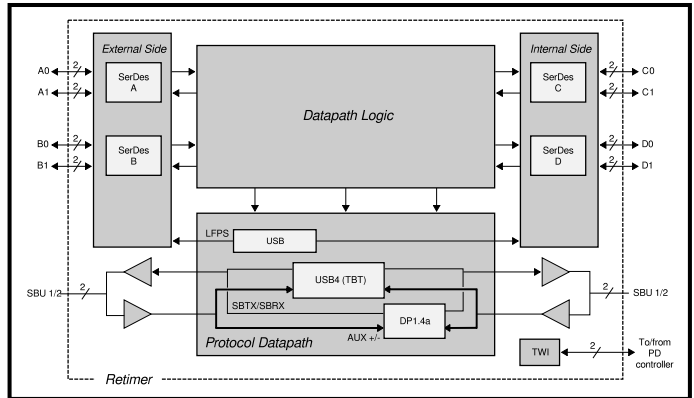
KB8001 Block Diagram
